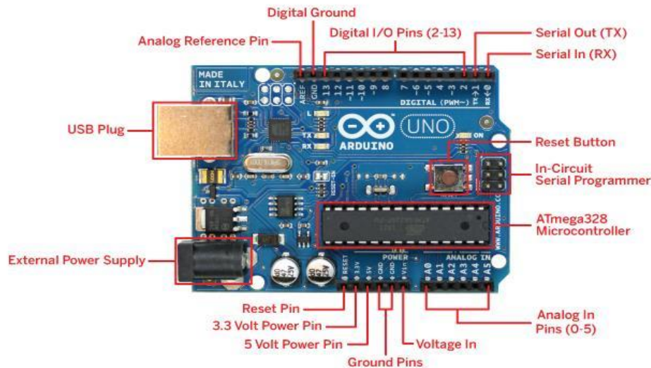
Figure 2.1 Schematic Diagram of Arduino 1
