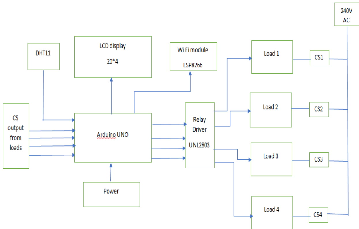
Figure 3.1 Block Diagram
