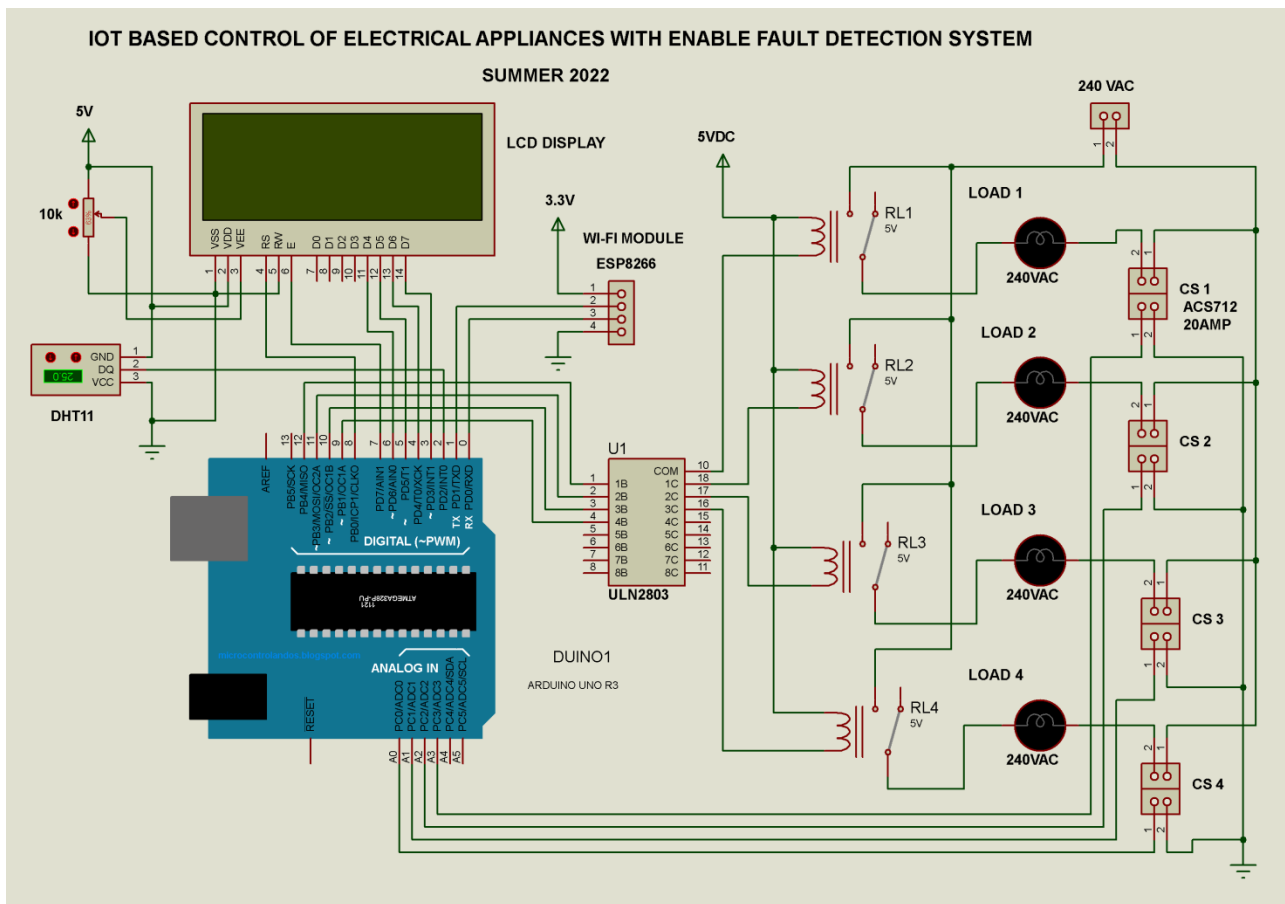
Figure 3.2 Circuit Diagram
