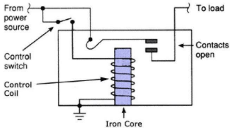
Figure 2.2 SPDT Relay 2
